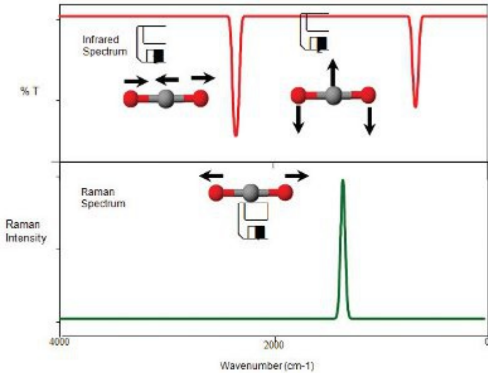
Figure 35. Schematic of CO 2 Raman and IR Spectra. “In gas phase spectra of CO 2 , two infrared modes are observed at 2350 and 667 cm -1 (red) and a single Raman band at ~1388 cm -1 (green). (The latter band is actually a doublet due to quantum mechanical resonance effects, which is beyond this discussion).” [48]
