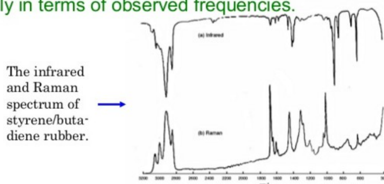
Figure 31. Complementary IR and Raman Spectroscopy. Infrared above; Raman below[45]
