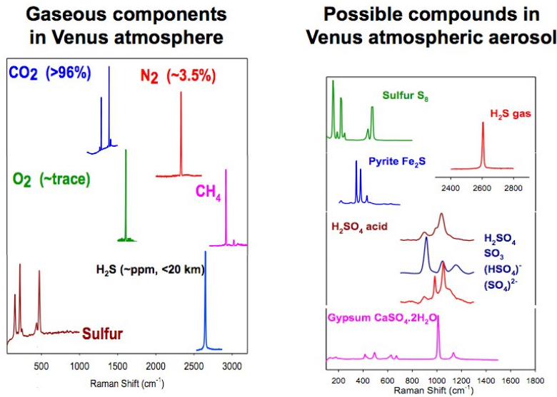
Figure 24. Venus Atmosphere ‘Raman Lines’ Showing molecules with their respective modes in Venus’s atmosphere. [31]
