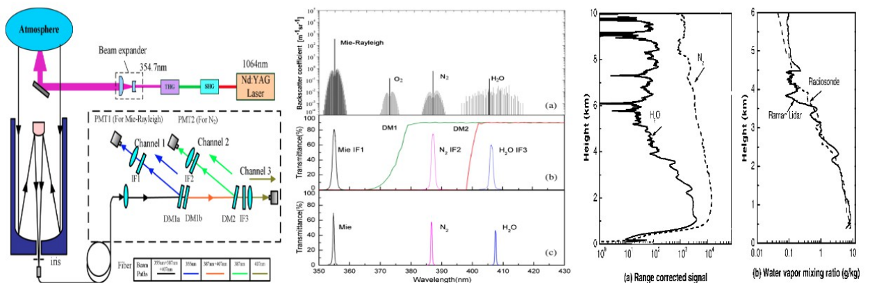
Figure 29. Raman Lidar [36]. Showing the ability of Raman Lidar to measure most atmospheric gases.
