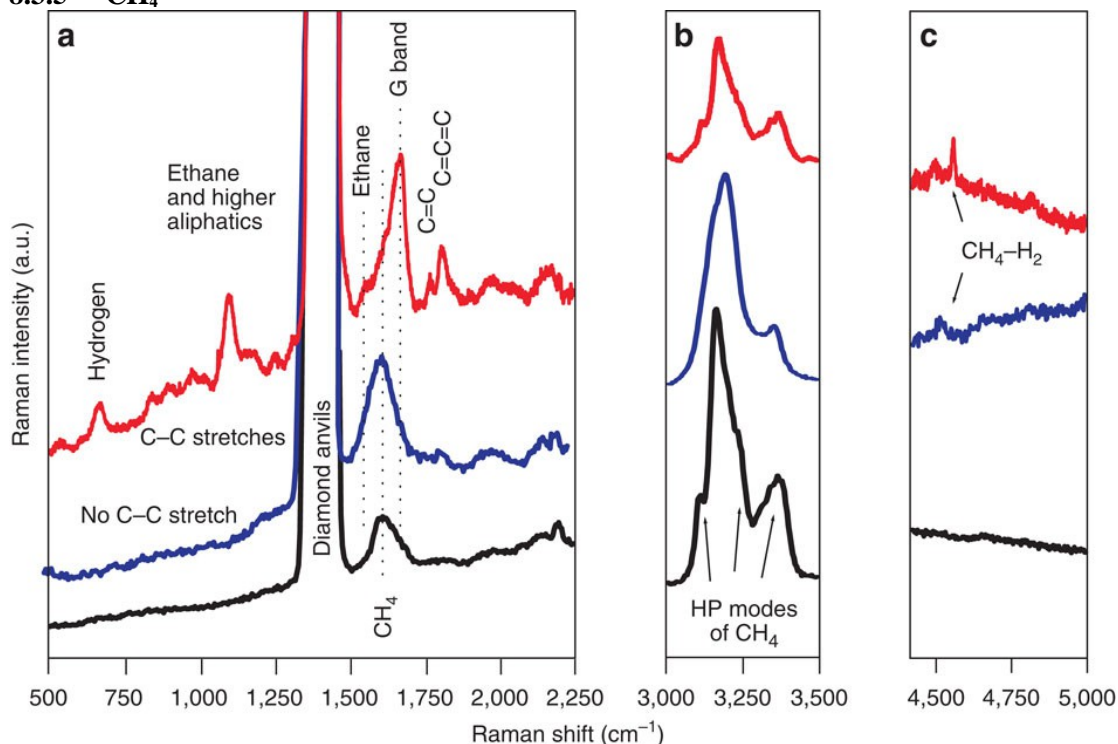
Figure 56. Synthesis in LH DAC at 48 GPa. Black line shows \text{CH}_4 Raman spectrum before heating. Blue line shows Raman spectrum collected at 1,445 K with evident \text{CH}_4 dissociation. Red line shows Raman spectrum of reaction products collected after heating to 2,000 K. The labels near the curves suggest the assignment of the Raman bands. HP modes of \text{CH}_4 refer to
