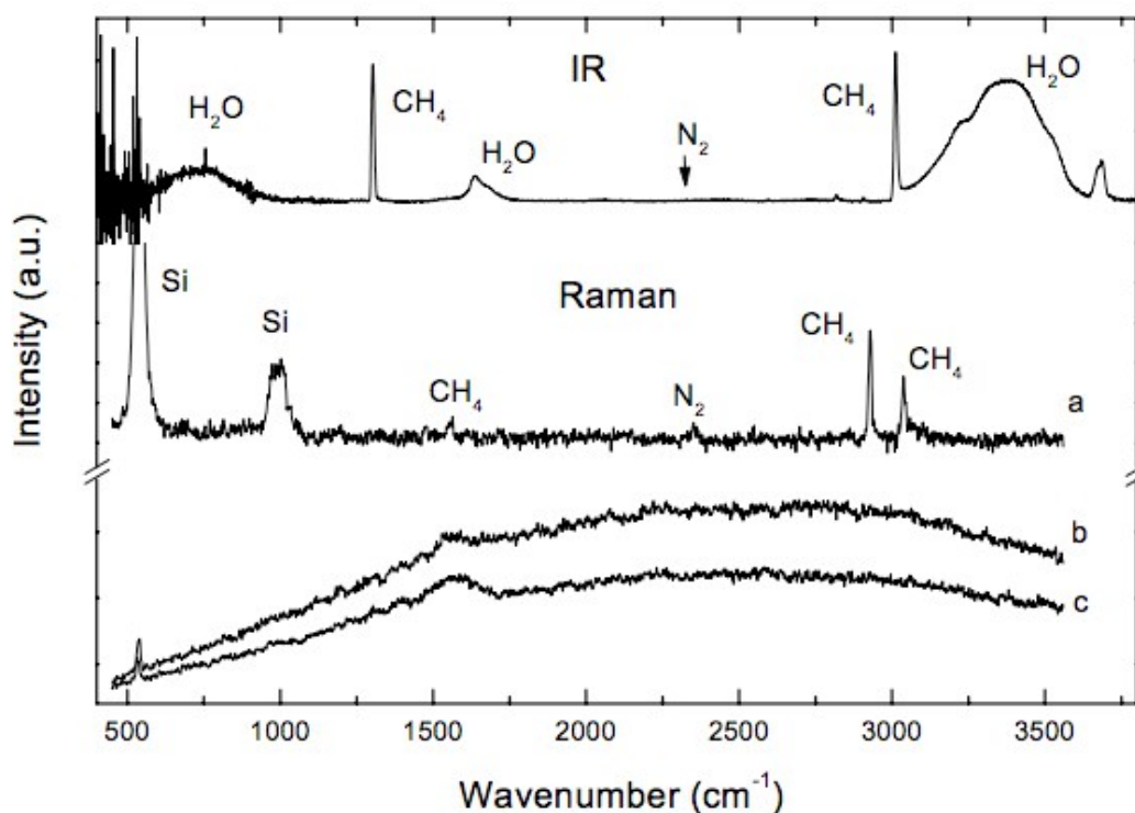
Figure 57. IR (top curve) and Raman spectra of the mixture H 2 O:CH 4 :N 2 before (curve a) and after (curves b and c, corresponding to doses of 378 eV/16 amu and 825 eV/16 amu respectively) irradiation with He + (30 keV) ions at low temperature (12 K). In spectra b and c the ice features are undetectable because of the intense fluorescence background. The arrow in the IR spectrum indicates the position of the N≡N symmetric stretching mode, which cannot be observed. Fig. 3 [94].
