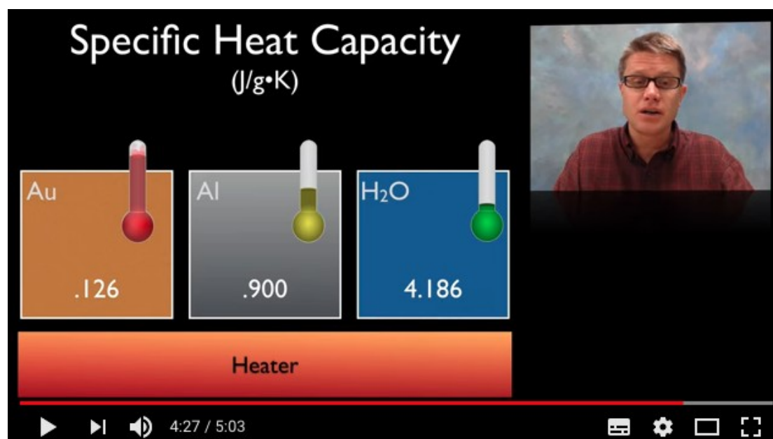
Figure 47. Specific Heat Capacity. The lower the heat capacity, the higher the temperature from single heat source.
